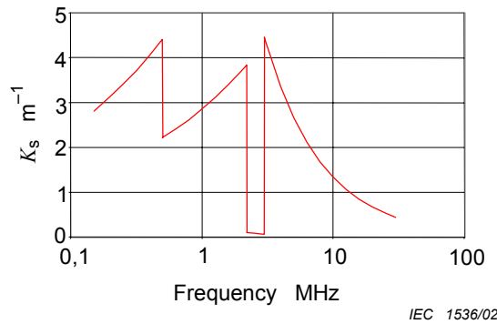
Figure 6-A2 – Factor K_s derived from the data in figure 6-A1 and equation (6-A4)
